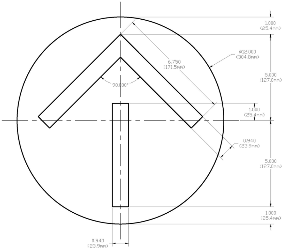
Figure 1: General Configuration of LED Vehicle Arrow Traffic Signal Icon (Dimensions are shown in inches and (mm))
